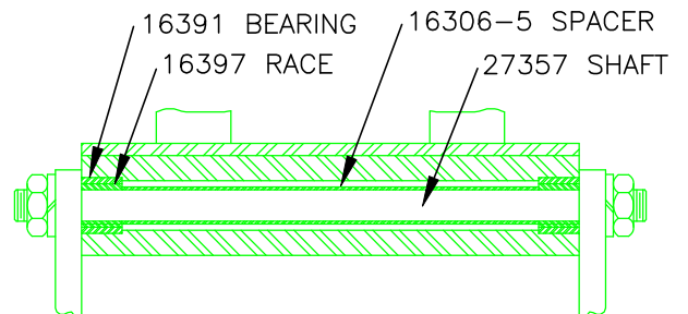
Section "G"
