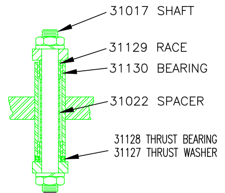
Section "D"
